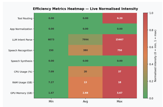
Fig. 10. Efficiency Heat Map. Min/Avg/Max normalised latency and resource usage per module; LLM inference dominates all other costs.
